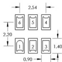
Pad Layout
