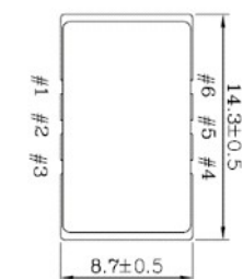
Package Outline Drawing
