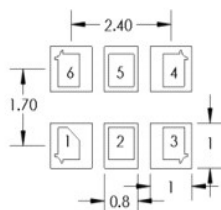
Pad Layout
