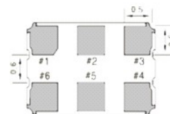
Package Outline Drawing
