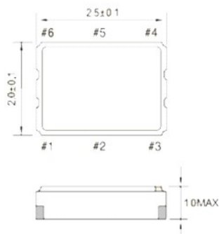
Package Outline Drawing
