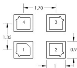
Pad Layout
