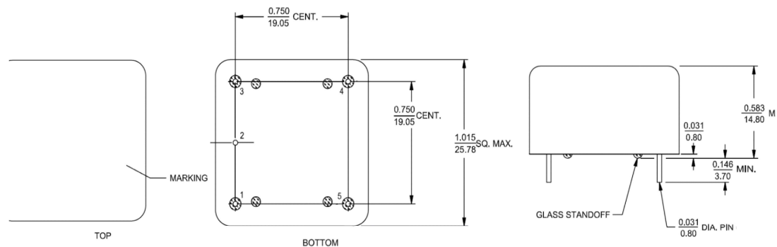
Package Outline Drawing
