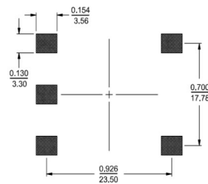
Pad Layout
