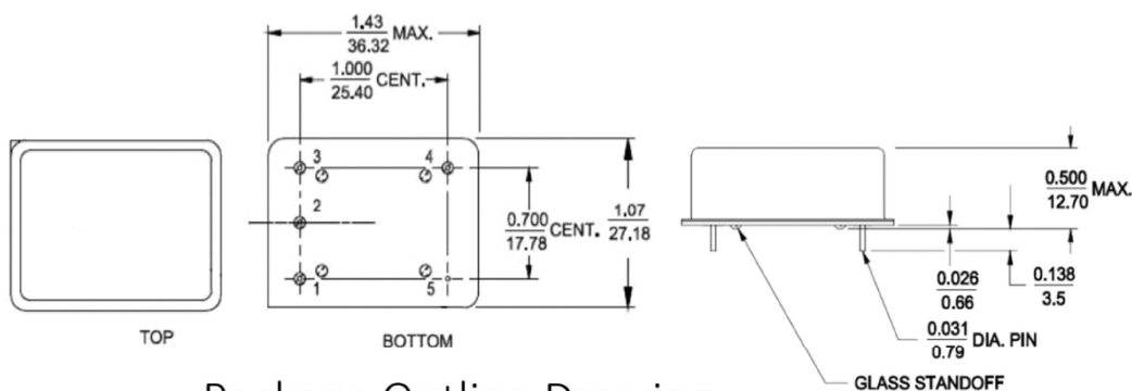
Package Outline Drawing
